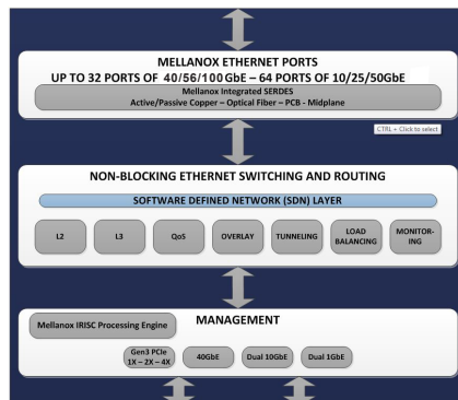
Figure 1. Mellanox Spectrum Architecture
