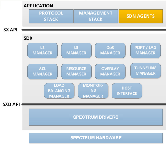
Figure 2. SDN-Optimized Software
